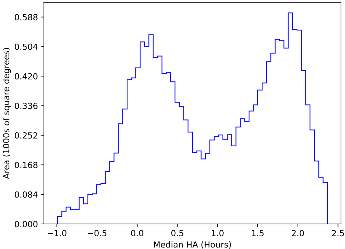
too_ignore_100_1v3.4_10yrs WFD u band: Median HA
