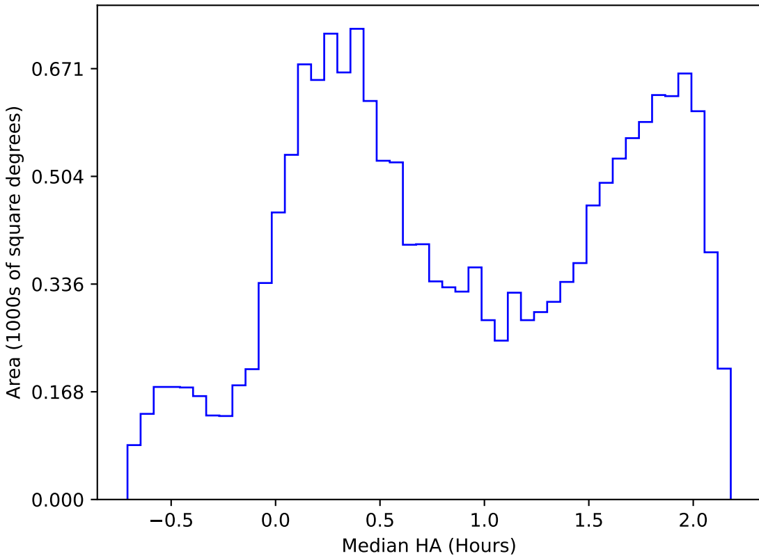
too_ignore_100_1v3.4_10yrs WFD r band: Median HA
