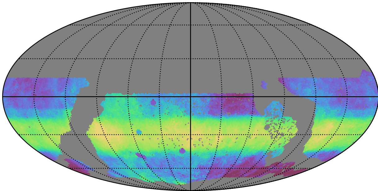
too_ignore_100_1v3.4_10yrs WFD i band: Median HA
