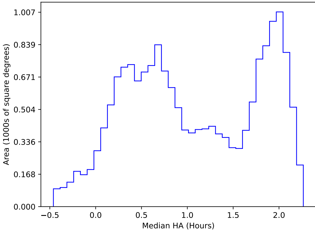
too_ignore_100_1v3.4_10yrs WFD i band: Median HA
