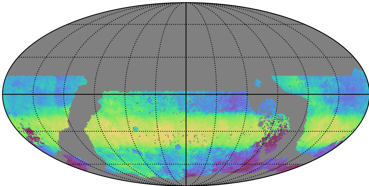
too_ignore_100_1v3.4_10yrs WFD g band: Median HA
