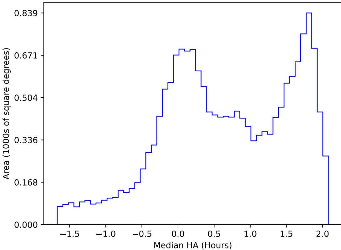
too_ignore_100_1v3.4_10yrs WFD g band: Median HA
