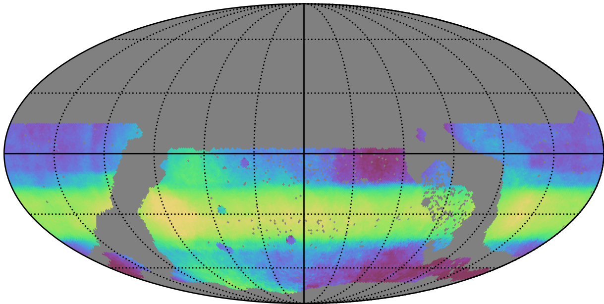
too_ignore_100_1v3.4_10yrs WFD all bands: Median HA
