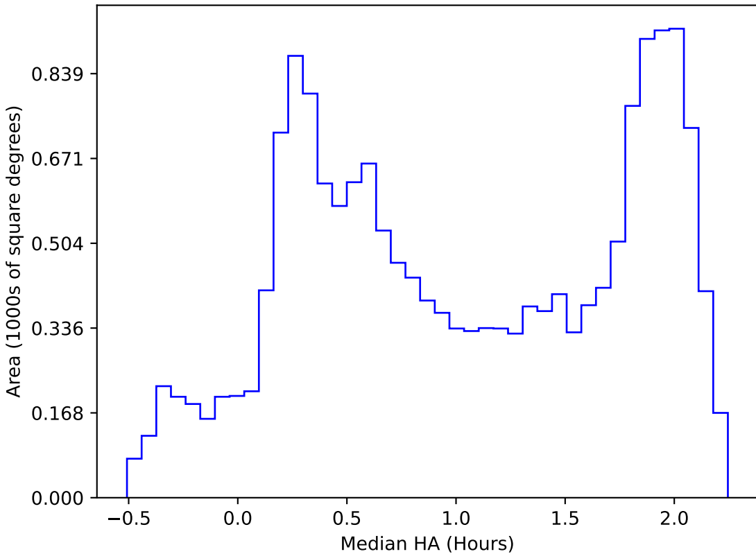
too_ignore_100_1v3.4_10yrs WFD all bands: Median HA
