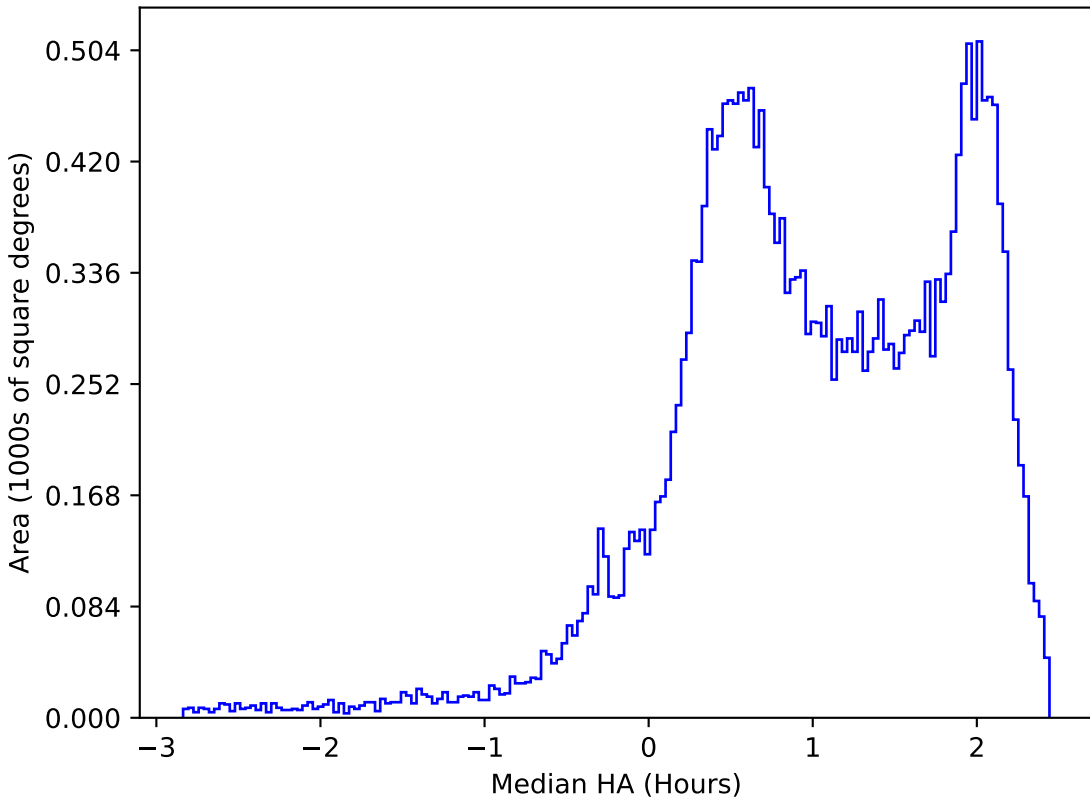
too_ignore_100_1v3.4_10yrs All sky z band: Median HA
