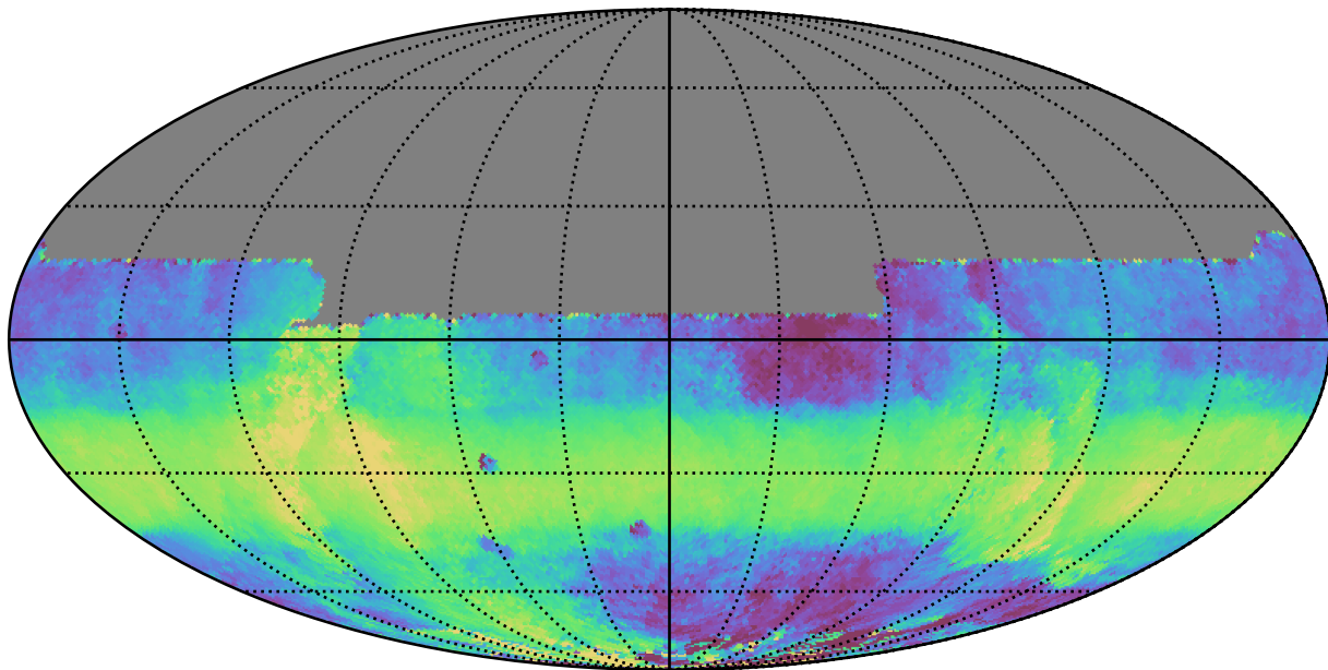
too_ignore_100_1v3.4_10yrs All sky y band: Median HA
