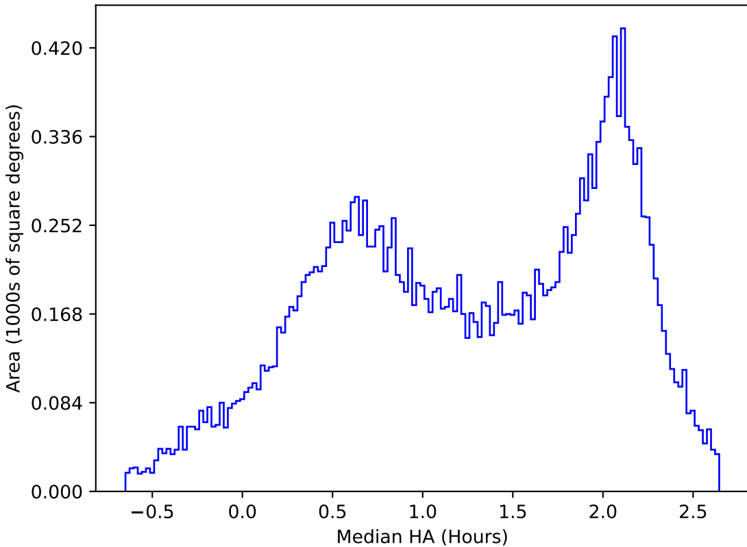
too_ignore_100_1v3.4_10yrs All sky y band: Median HA
