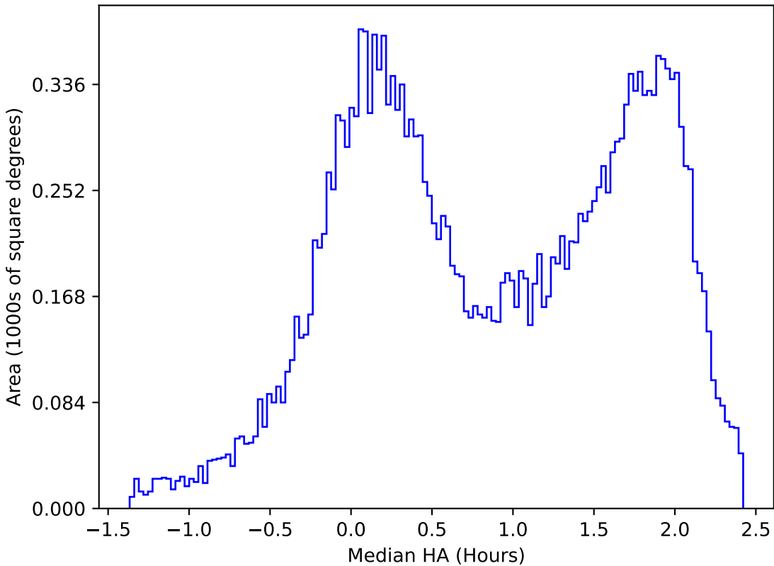
too_ignore_100_1v3.4_10yrs All sky u band: Median HA
