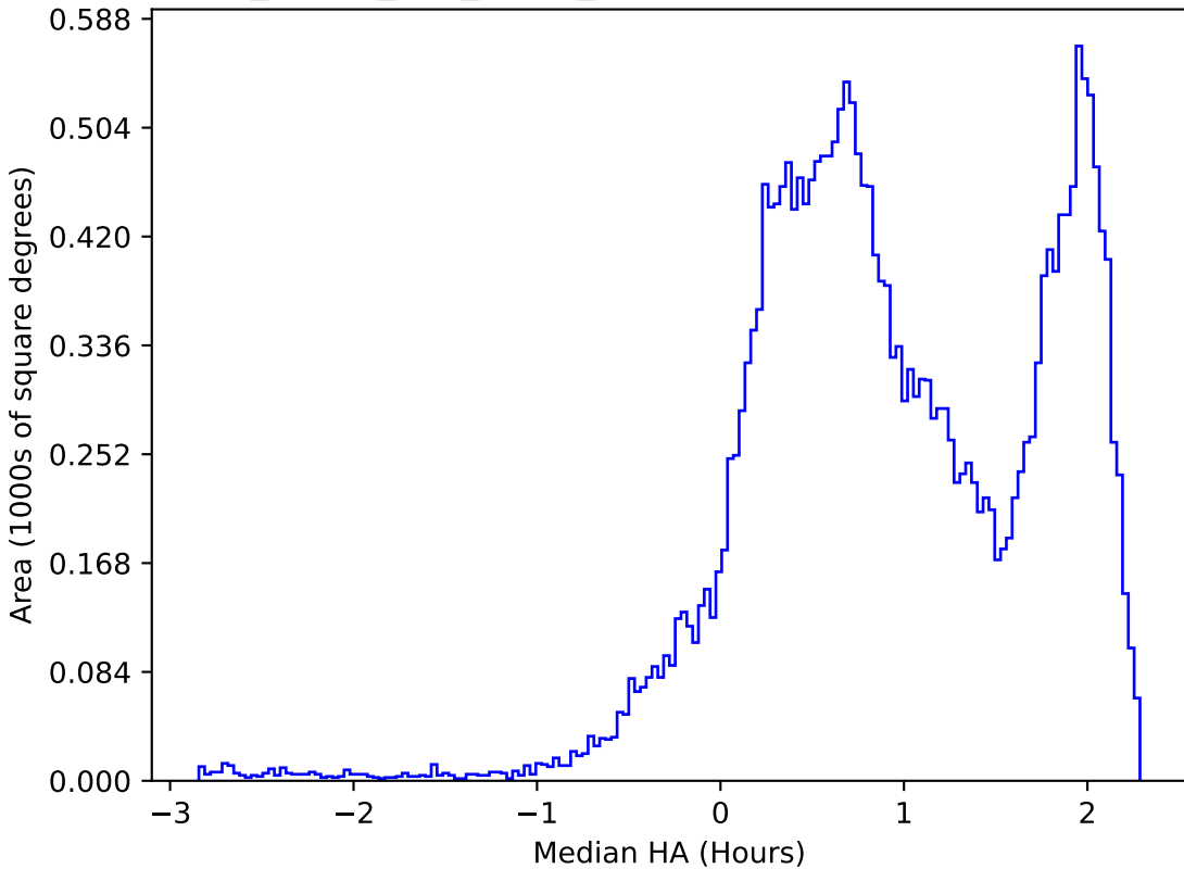
too_ignore_100_1v3.4_10yrs All sky i band: Median HA
