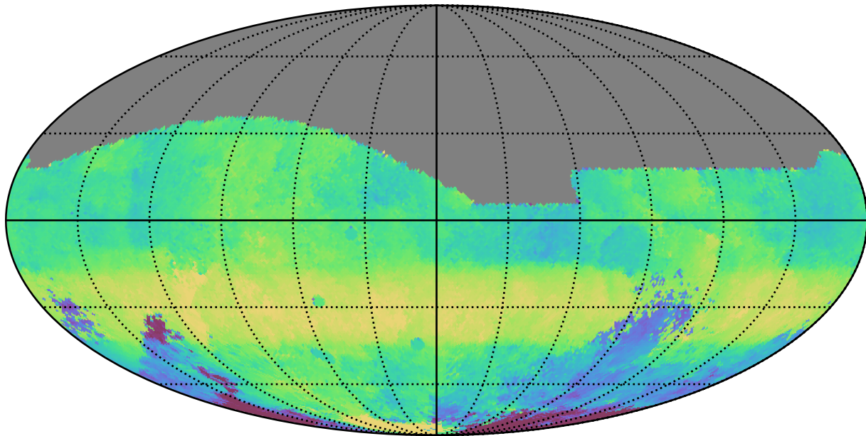
too_ignore_100_1v3.4_10yrs All sky g band: Median HA
