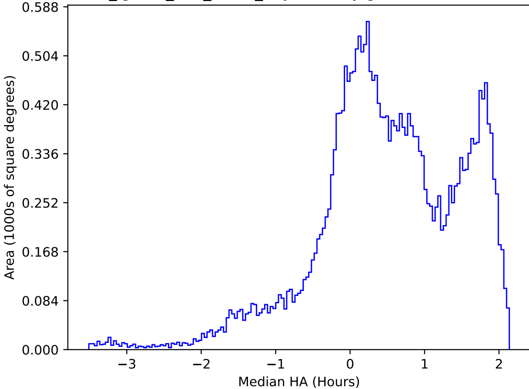
too_ignore_100_1v3.4_10yrs All sky g band: Median HA
