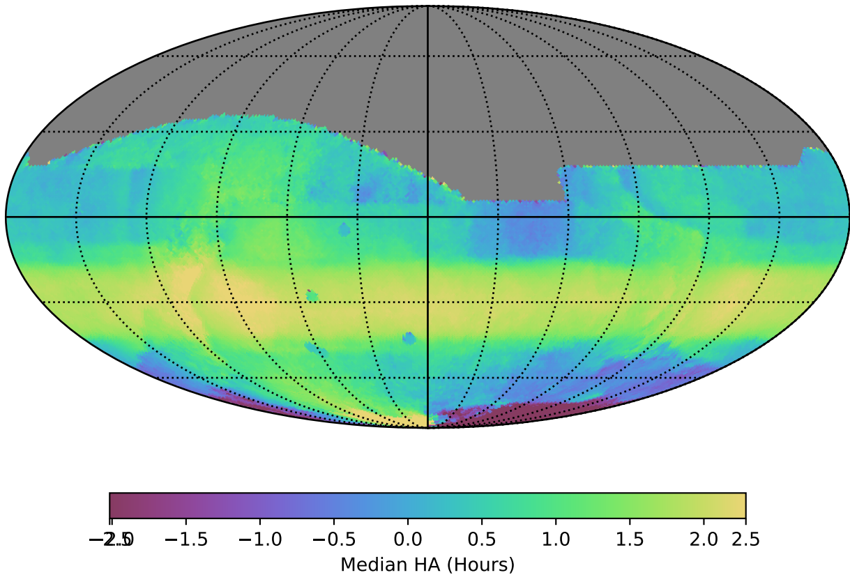
too_ignore_100_1v3.4_10yrs All sky all bands: Median HA
