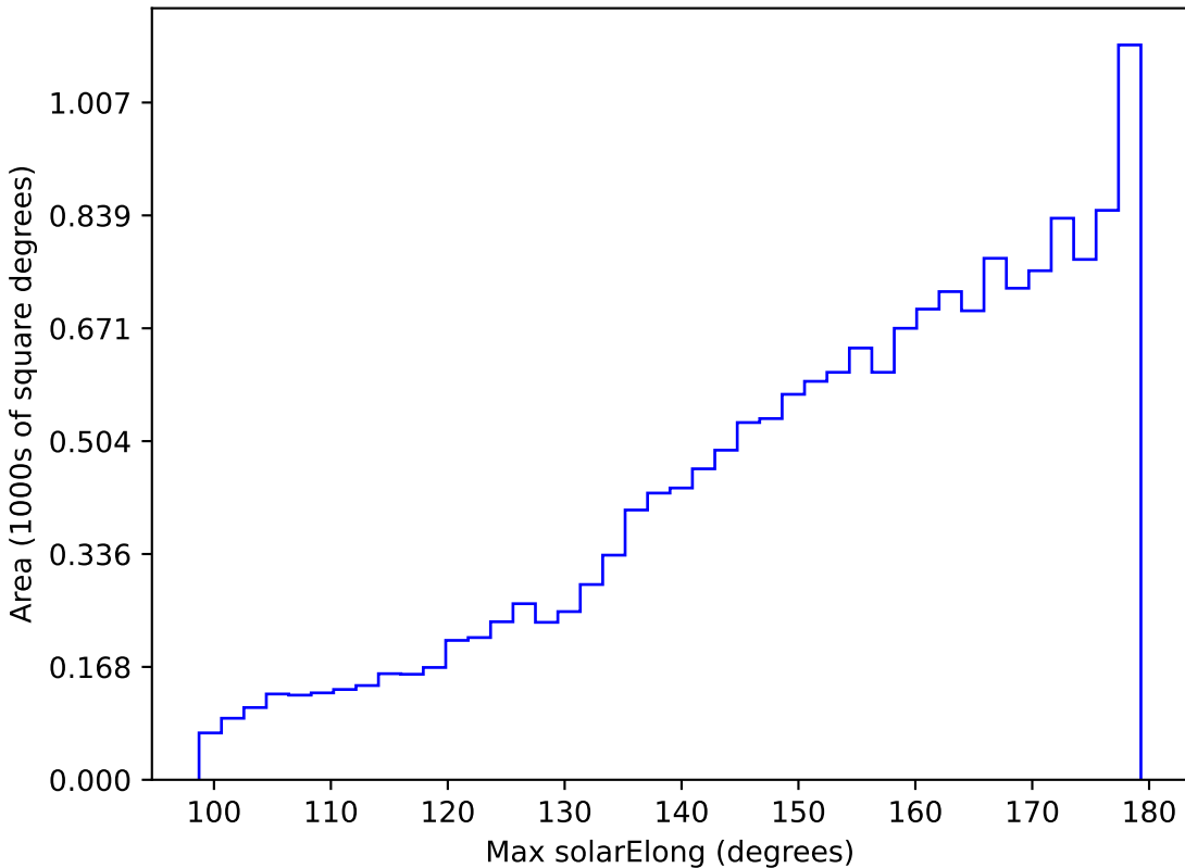
too_ignore_100_1v3.4_10yrs WFD z band: Max solarElong
