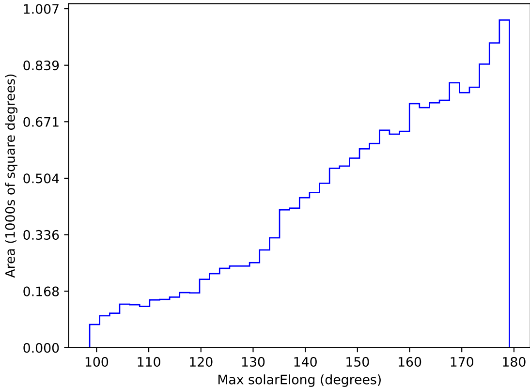
too_ignore_100_1v3.4_10yrs WFD y band: Max solarElong
