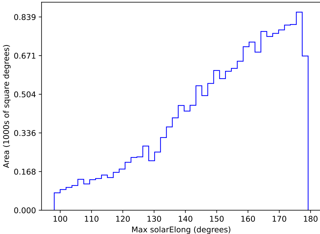
too_ignore_100_1v3.4_10yrs WFD u band: Max solarElong
