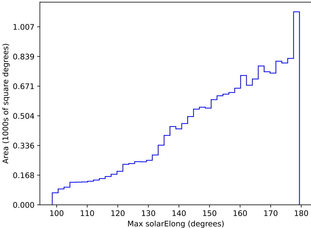
too_ignore_100_1v3.4_10yrs WFD r band: Max solarElong
