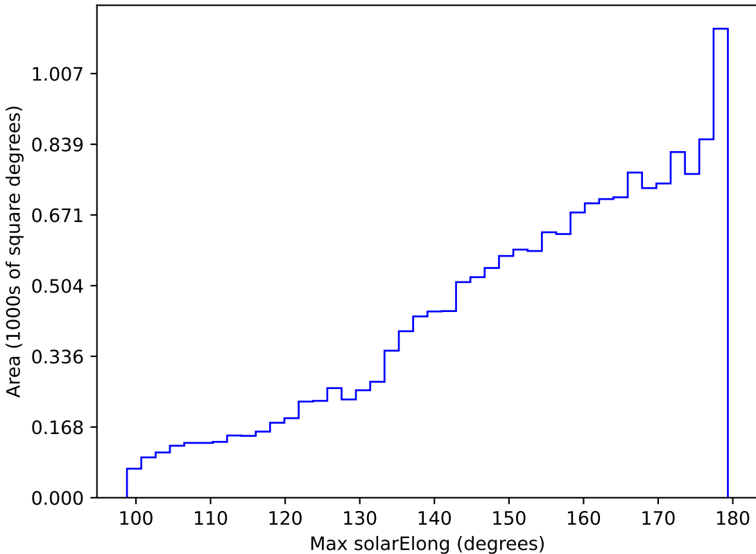
too_ignore_100_1v3.4_10yrs WFD i band: Max solarElong
