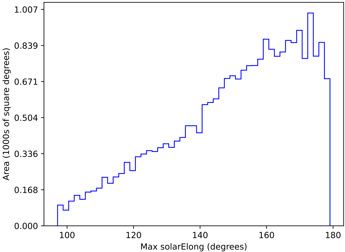
too_ignore_100_1v3.4_10yrs All sky u band: Max solarElong
