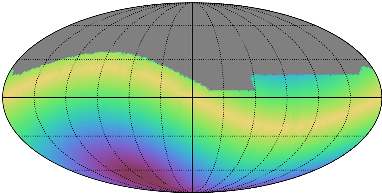
too_ignore_100_1v3.4_10yrs All sky r band: Max solarElong
