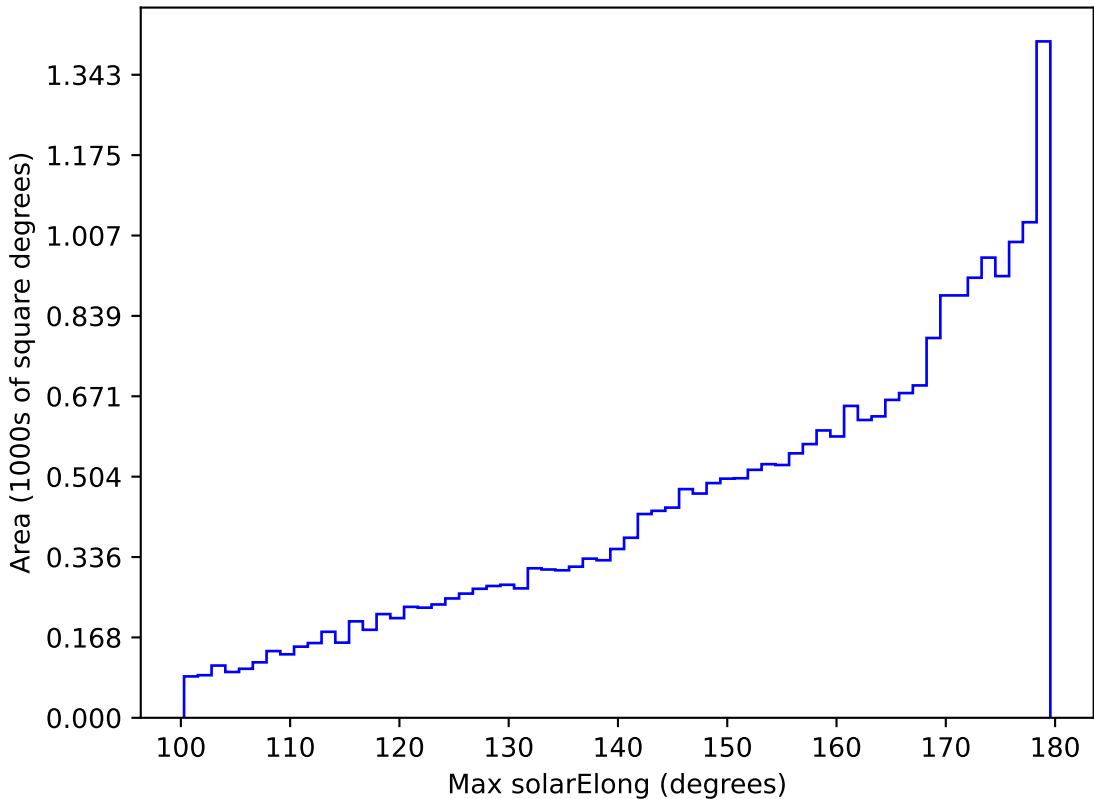
too_ignore_100_1v3.4_10yrs All sky all bands: Max solarElong
