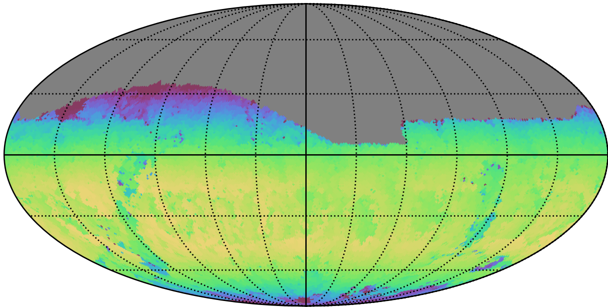
too_ignore_100_1v3.4_10yrs Yr 1 z band: Max skyBrightness
