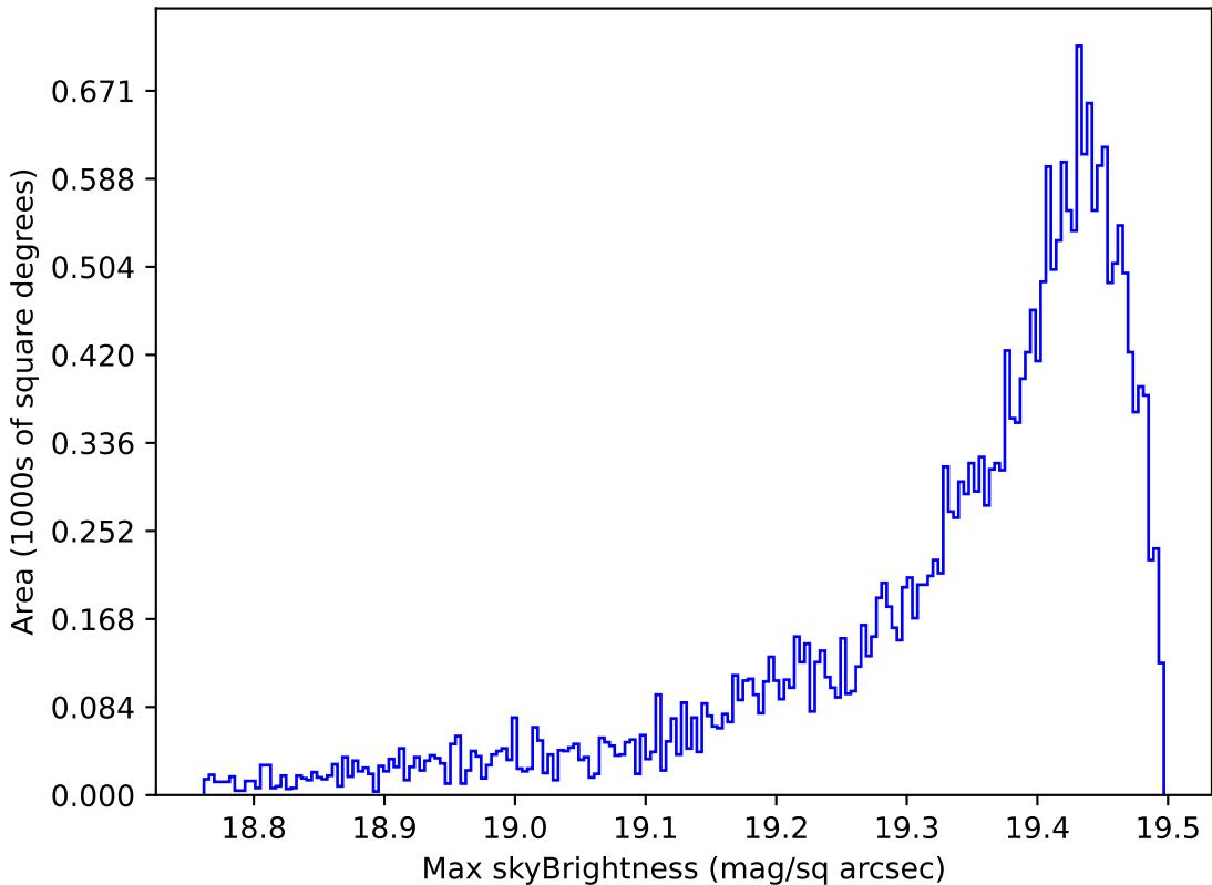
too_ignore_100_1v3.4_10yrs Yr 1 z band: Max skyBrightness
