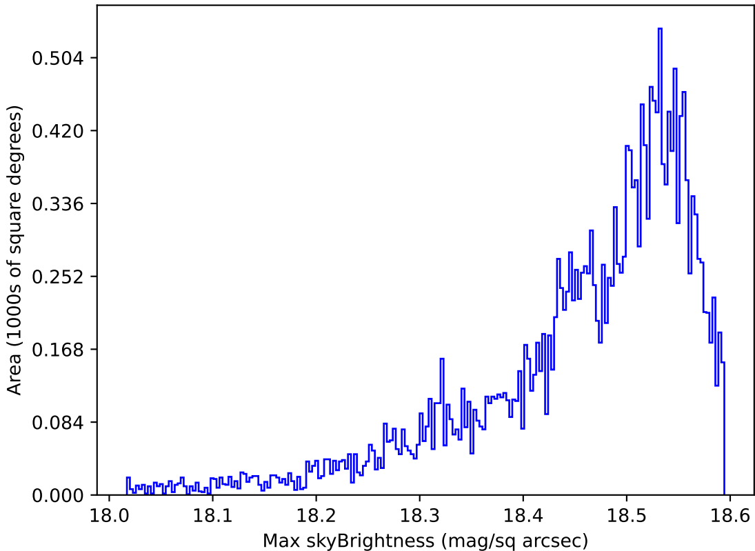
too_ignore_100_1v3.4_10yrs Yr 1 y band: Max skyBrightness
