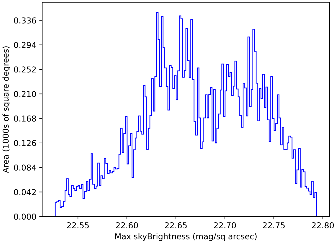
too_ignore_100_1v3.4_10yrs Yr 1 u band: Max skyBrightness
