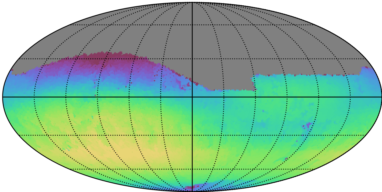
too_ignore_100_1v3.4_10yrs Yr 1 r band: Max skyBrightness
