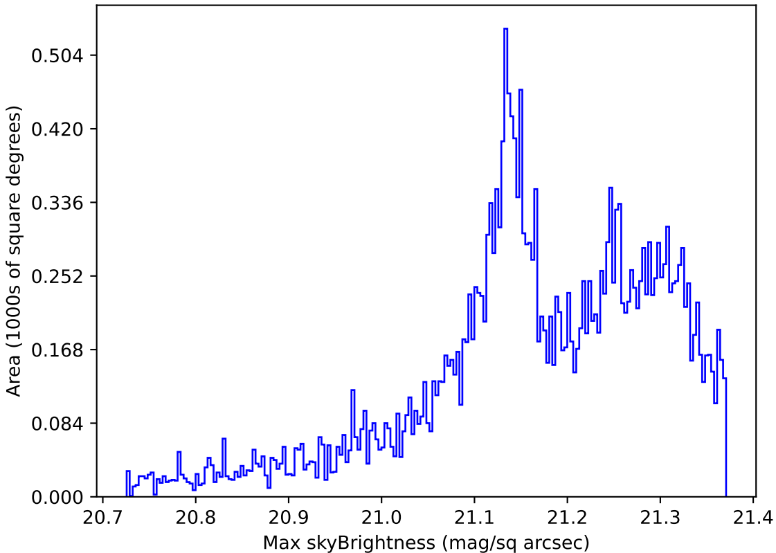
too_ignore_100_1v3.4_10yrs Yr 1 r band: Max skyBrightness
