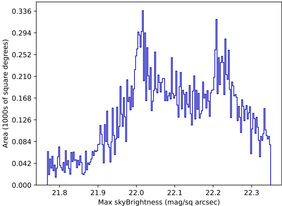
too_ignore_100_1v3.4_10yrs Yr 1 g band: Max skyBrightness
