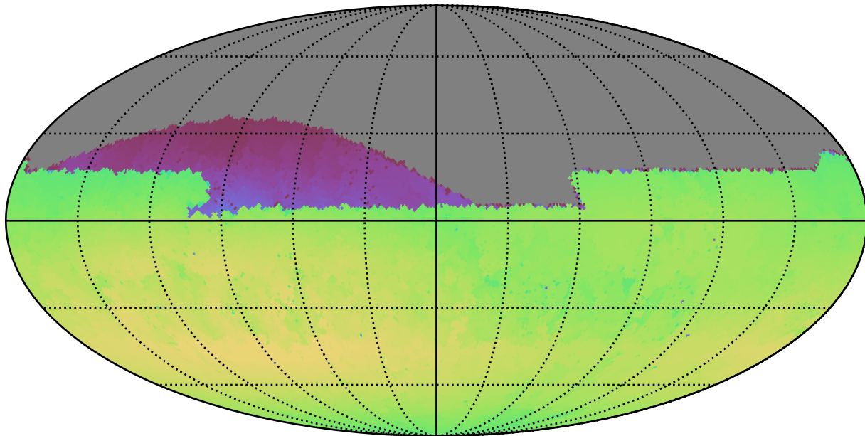
too_ignore_100_1v3.4_10yrs Yr 1 all bands: Max skyBrightness
