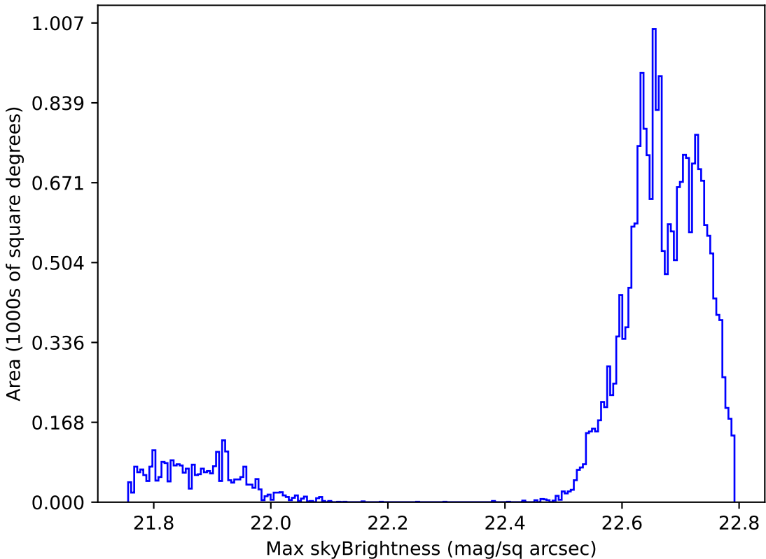
too_ignore_100_1v3.4_10yrs Yr 1 all bands: Max skyBrightness
