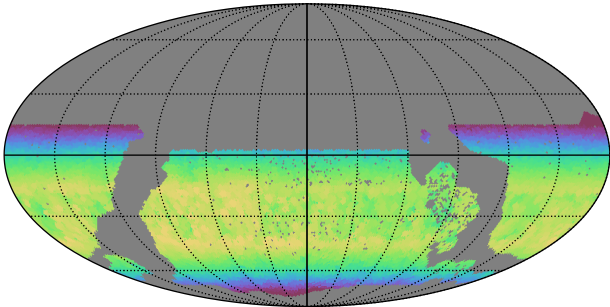
too_ignore_100_1v3.4_10yrs WFD y band: Max skyBrightness
