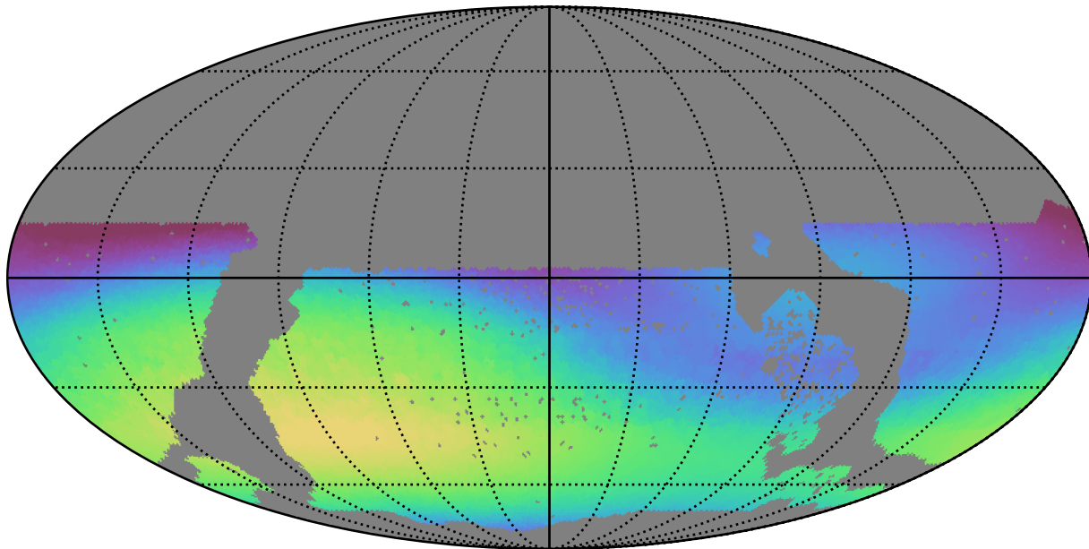
too_ignore_100_1v3.4_10yrs WFD r band: Max skyBrightness
