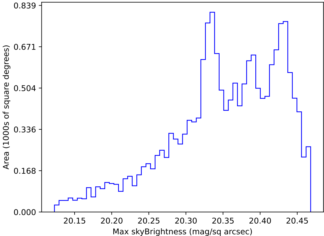
too_ignore_100_1v3.4_10yrs WFD i band: Max skyBrightness
