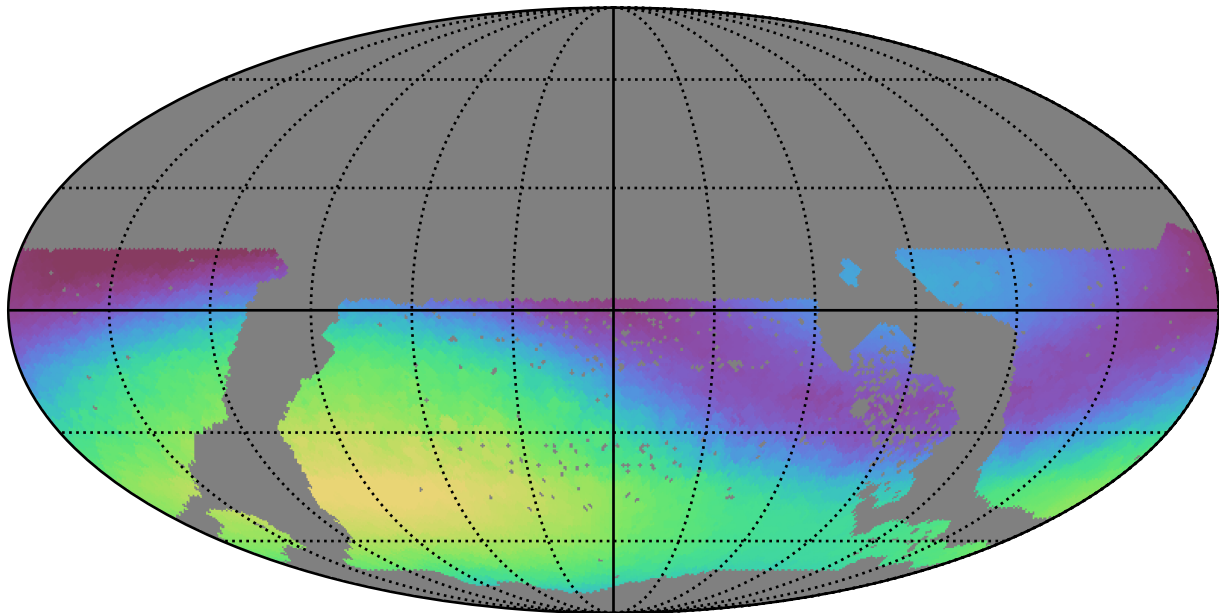
too_ignore_100_1v3.4_10yrs WFD g band: Max skyBrightness
