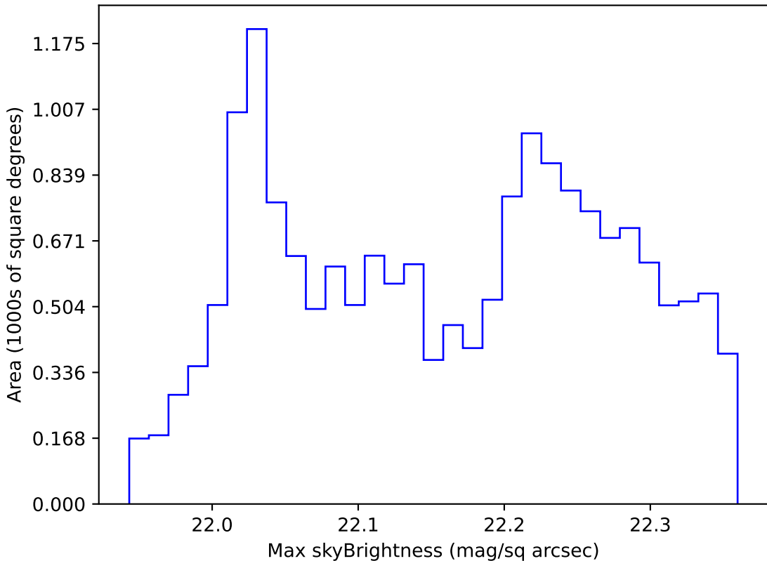
too_ignore_100_1v3.4_10yrs WFD g band: Max skyBrightness
