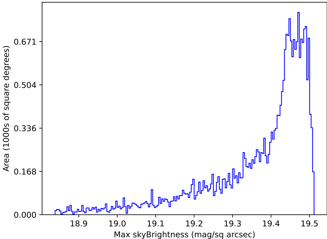
too_ignore_100_1v3.4_10yrs All sky z band: Max skyBrightness
