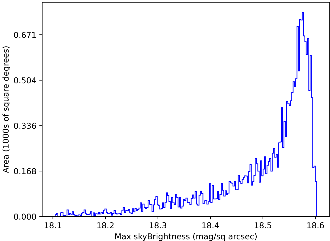
too_ignore_100_1v3.4_10yrs All sky y band: Max skyBrightness
