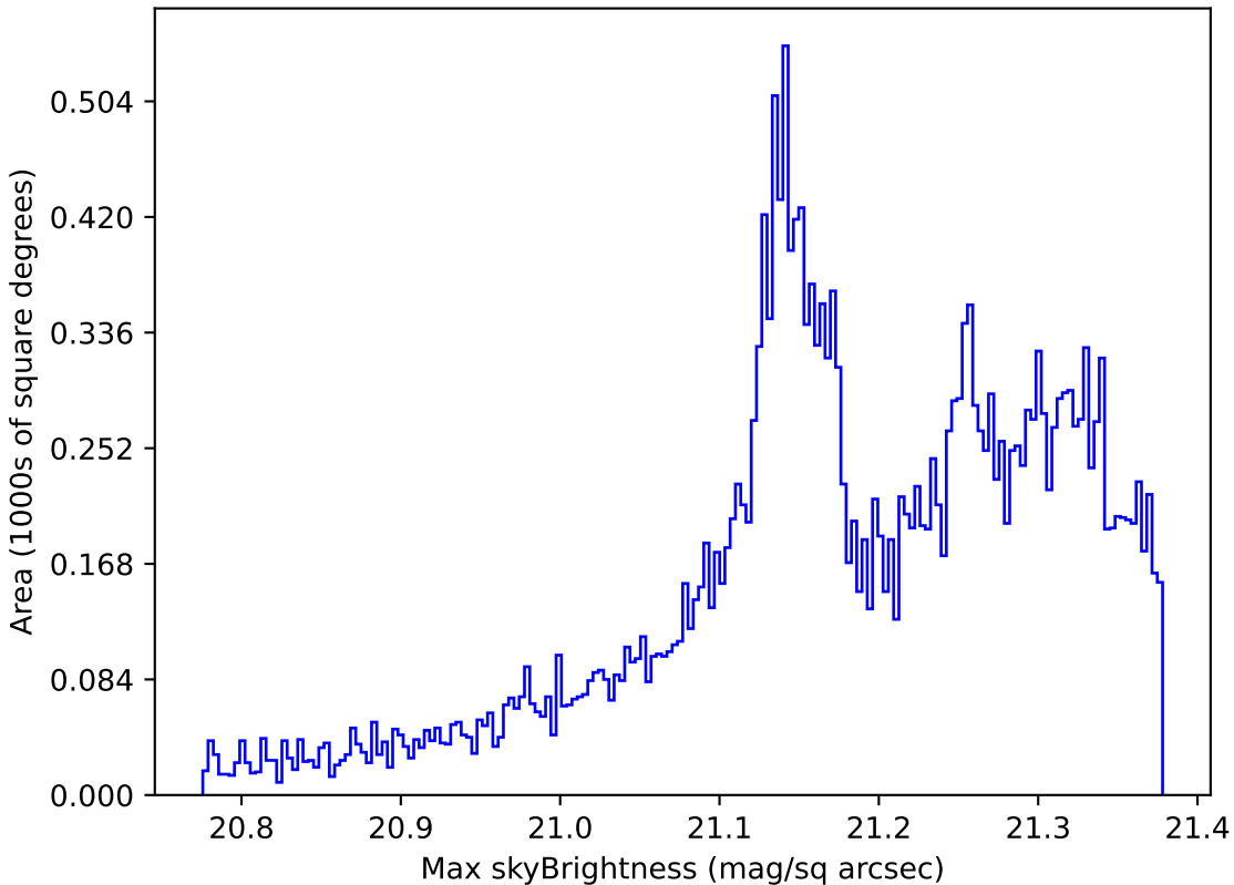
too_ignore_100_1v3.4_10yrs All sky r band: Max skyBrightness
