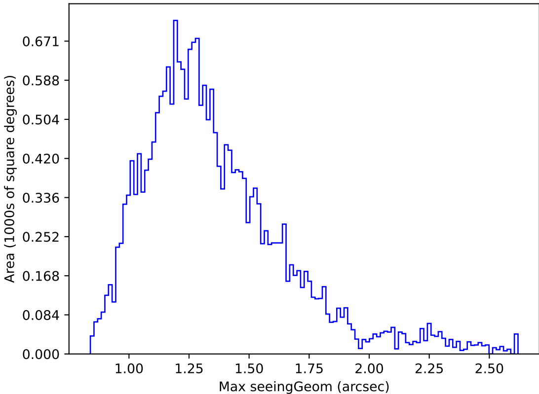
too_ignore_100_1v3.4_10yrs Yr 1 u band: Max seeingGeom
