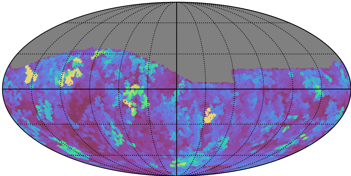
too_ignore_100_1v3.4_10yrs Yr 1 i band: Max seeingGeom
