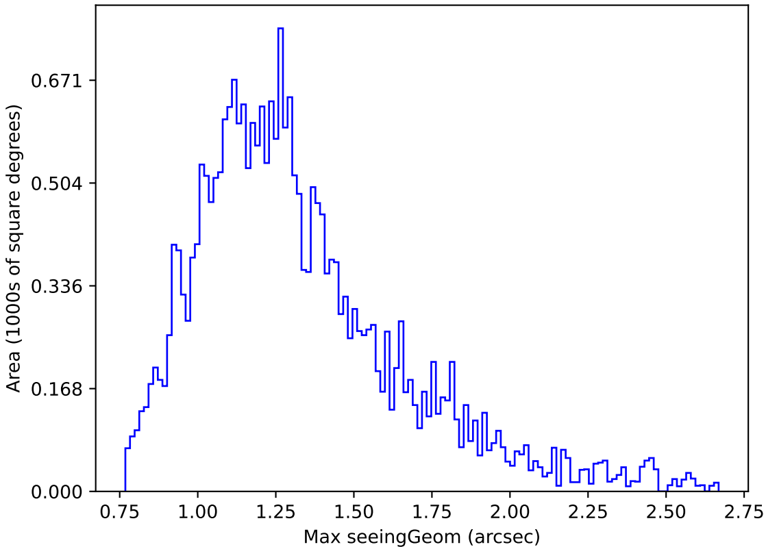
too_ignore_100_1v3.4_10yrs Yr 1 g band: Max seeingGeom
