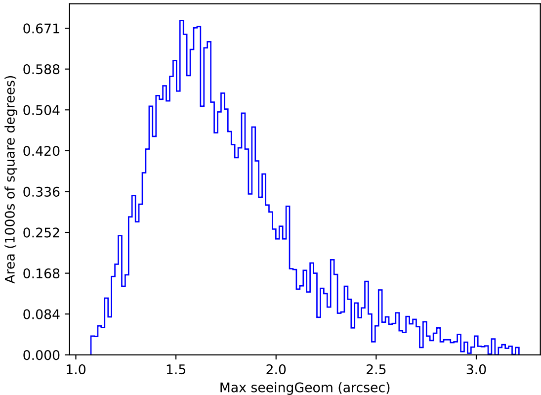
too_ignore_100_1v3.4_10yrs Yr 1 all bands: Max seeingGeom
