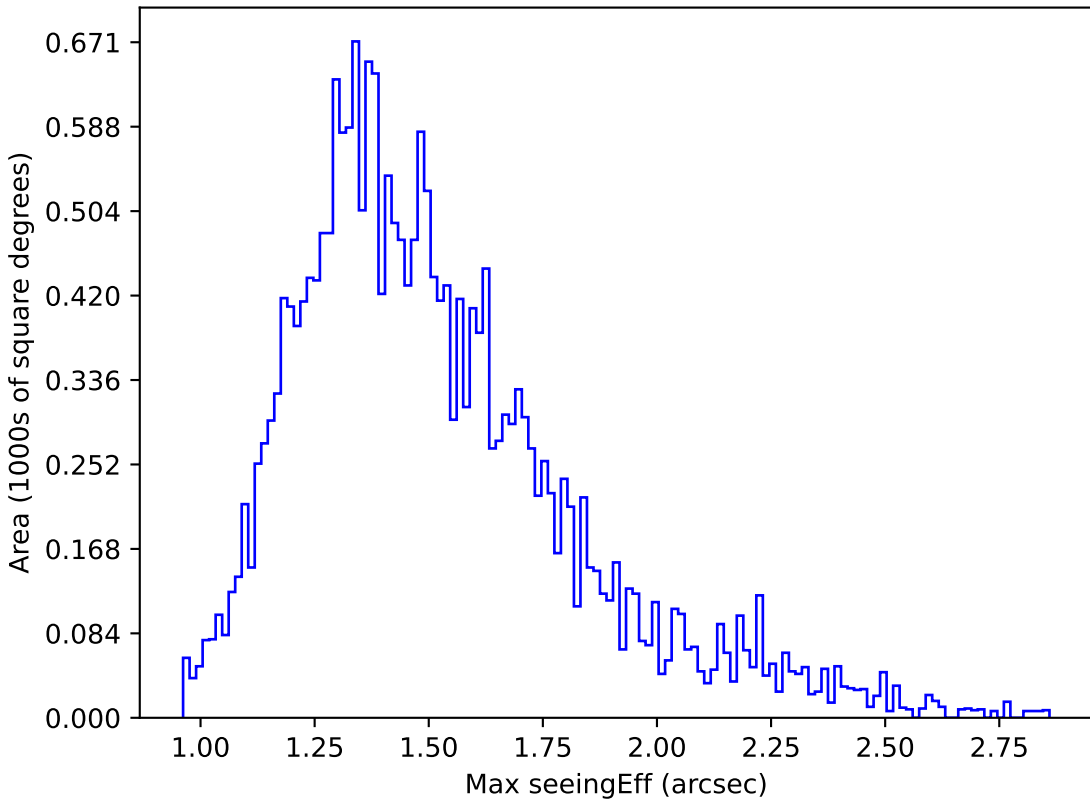
too_ignore_100_1v3.4_10yrs Yr 1 y band: Max seeingEff
