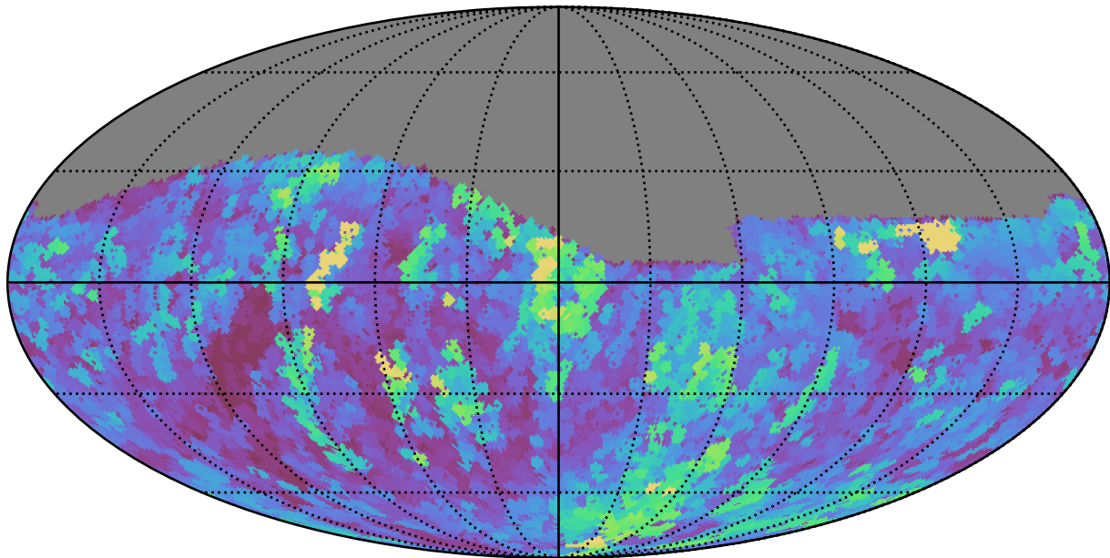
too_ignore_100_1v3.4_10yrs Yr 1 r band: Max seeingEff
