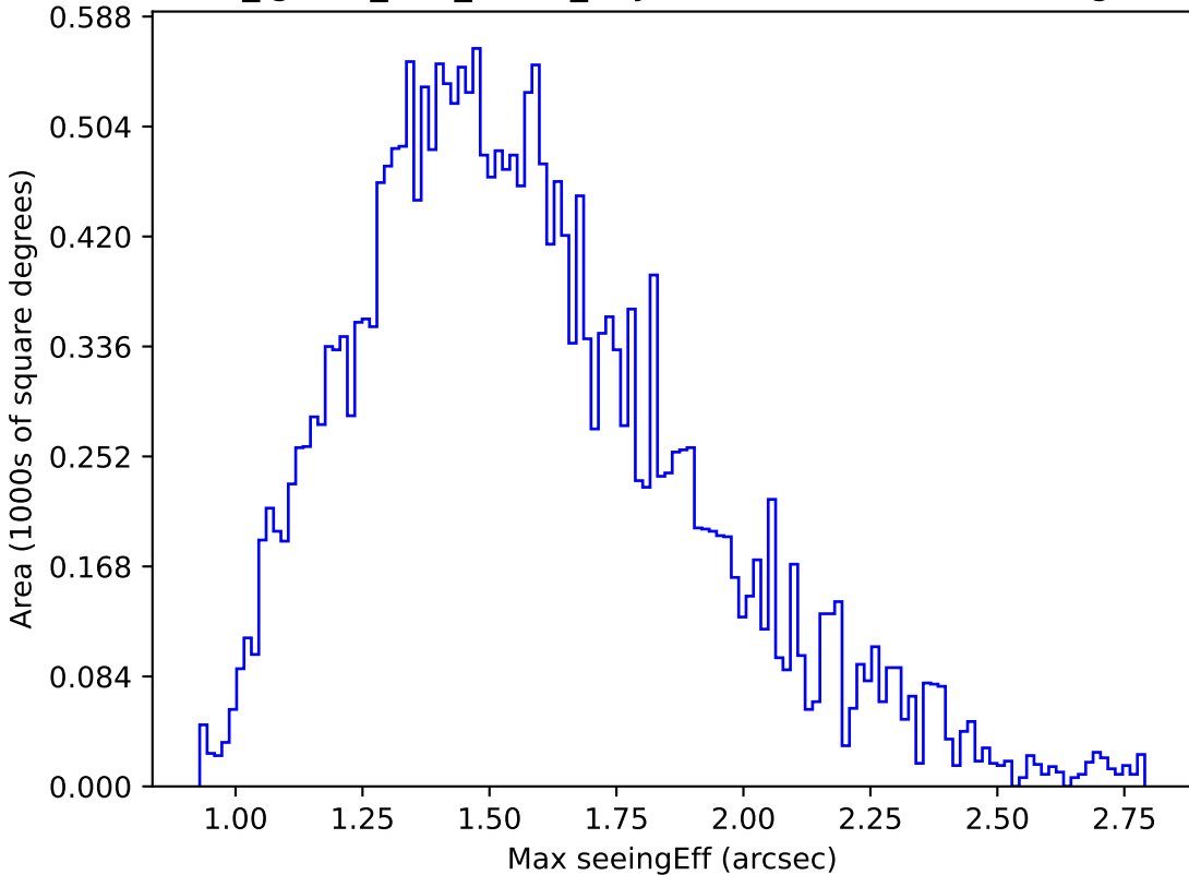
too_ignore_100_1v3.4_10yrs Yr 1 r band: Max seeingEff
