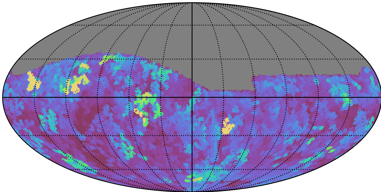
too_ignore_100_1v3.4_10yrs Yr 1 i band: Max seeingEff
