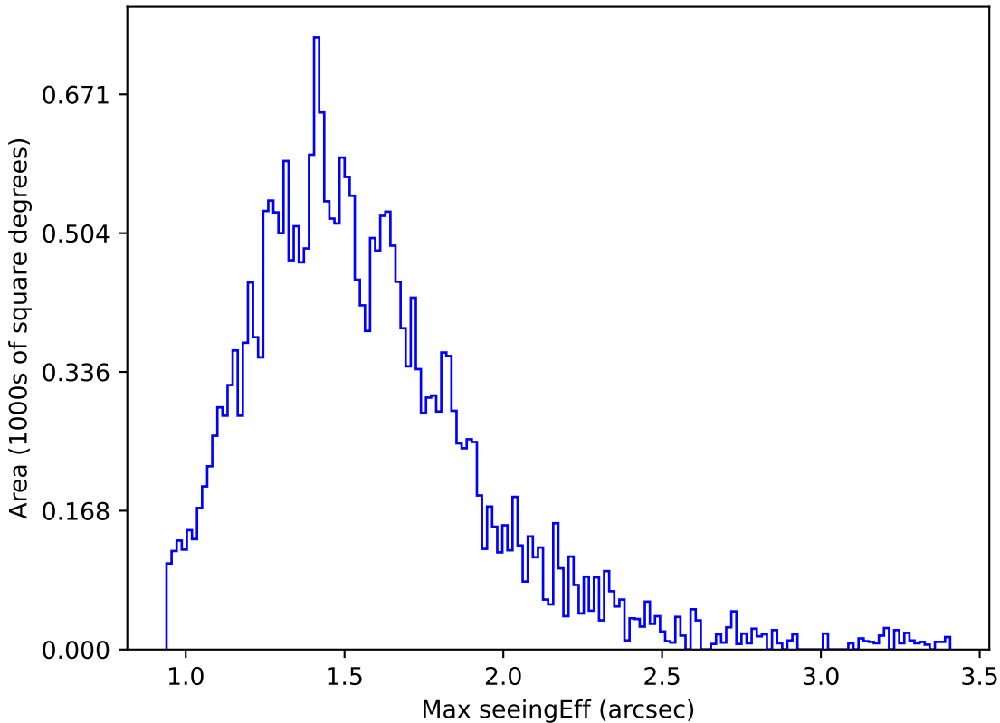
too_ignore_100_1v3.4_10yrs Yr 1 i band: Max seeingEff
